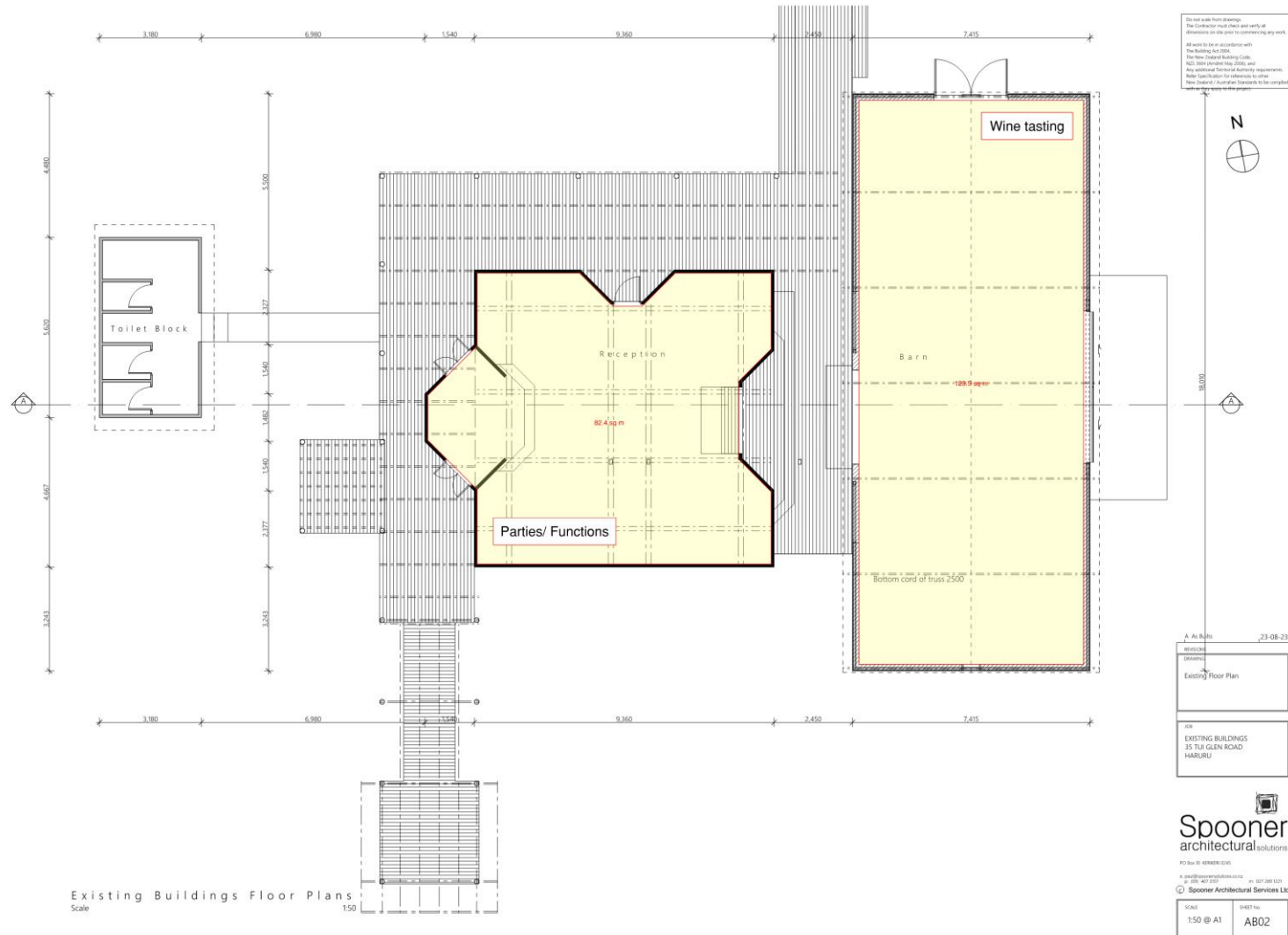
Figure 5: Floor plan
